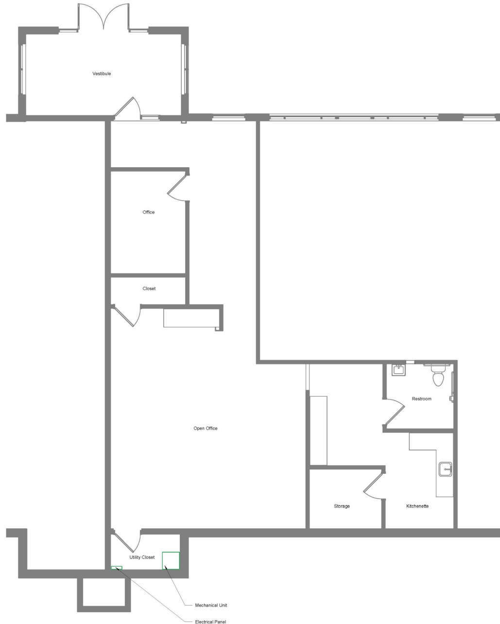
A7 Suite 102 - Floor Plan SC02 1/4" = 1'-0"
